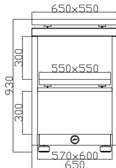
3 LEVELS, 3 COMPONENTS RACK CODE: SS-WBR-550 1+1+1
