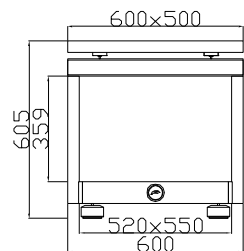
2 LEVELS, 2 COMPONENTS RACK CODE: SS-WBR-500 1+1
