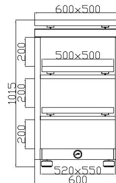
4 LEVELS, 4 COMPONENTS RACK CODE: SS-WBR-500 1+1+1+1
