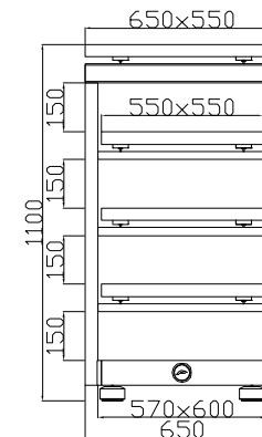
5 LEVELS, 5 COMPONENTS RACK CODE: SS-WBR-550 1+1+1+1+1
