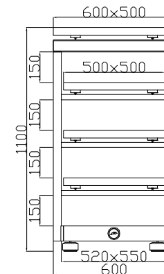
5 LEVELS, 5 COMPONENTS RACK CODE: SS-WBR-500 1+1+1+1+1
