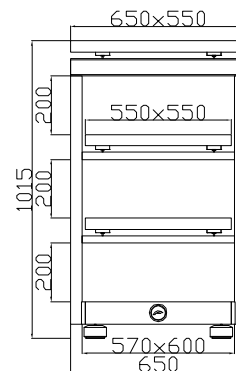
4 LEVELS, 4 COMPONENTS RACK CODE: SS-WBR-550 1+1+1+1
